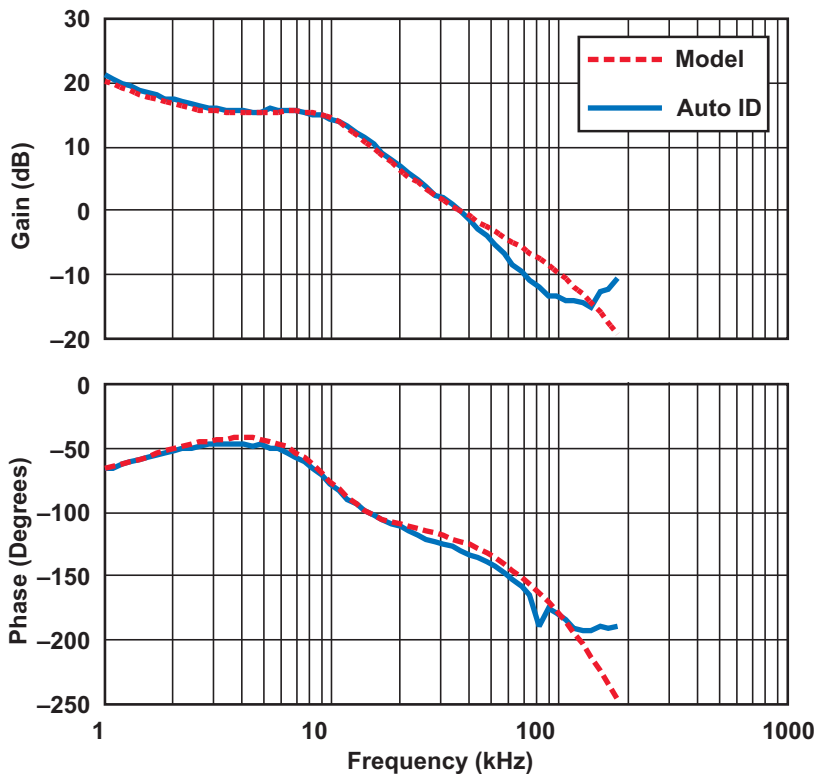
Fig. 27. Bode plot measured with Auto-ID versus model.
