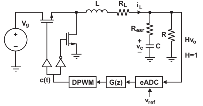
Fig. 5. Voltage-mode, closed-loop buck converter.
