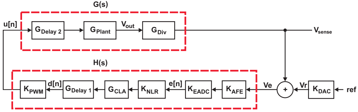
Fig. 3. Closed-loop block diagram.
