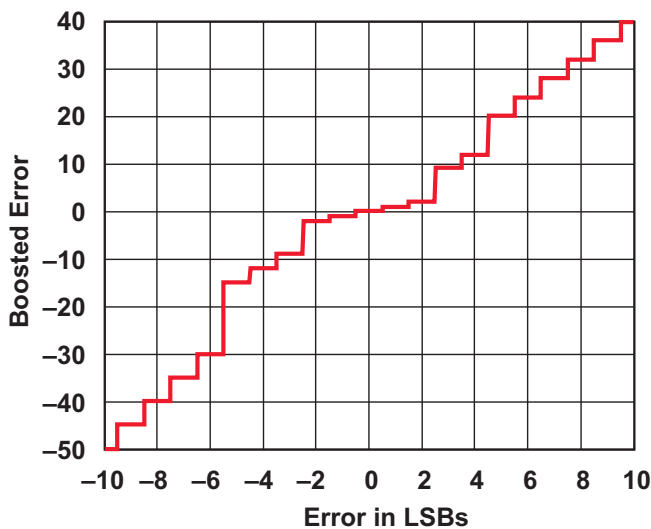
a. Transfer function after nonlinear gain.
