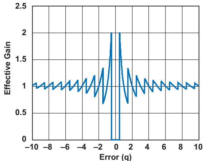
b. ADC gain due to quantization.
