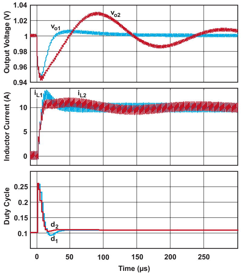
Fig. 15. Simulation results for a load transient of 1 to 10 A.
