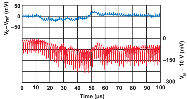
Fig. 37. The step-up load-transient response.
