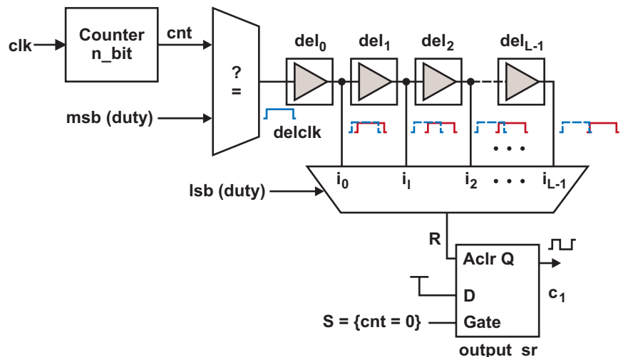
Fig. 22. Hybrid DPWM with external clock.
