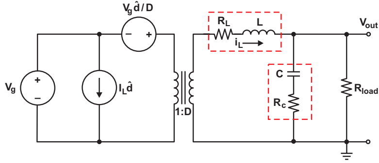
Fig. 4. Small-signal model of a buck converter with losses.
