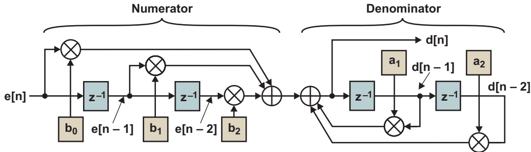
Fig. 10. Direct-form digital-filter implementation.
