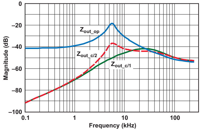
Fig. 14. The magnitude response of the open-loop and closed-loop output impedance.
