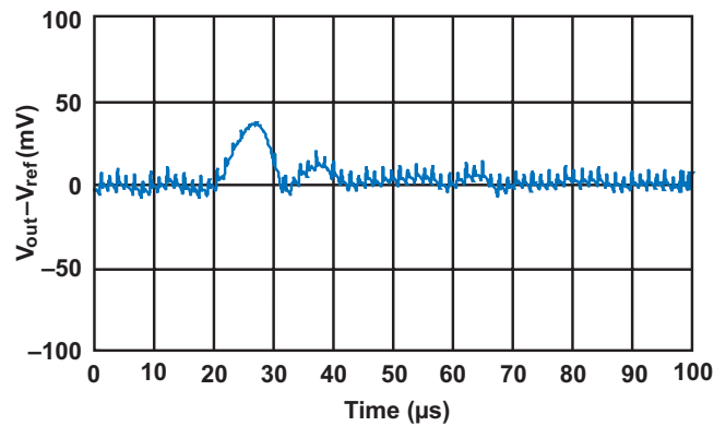
Fig. 36. The step-down load-transient response.
