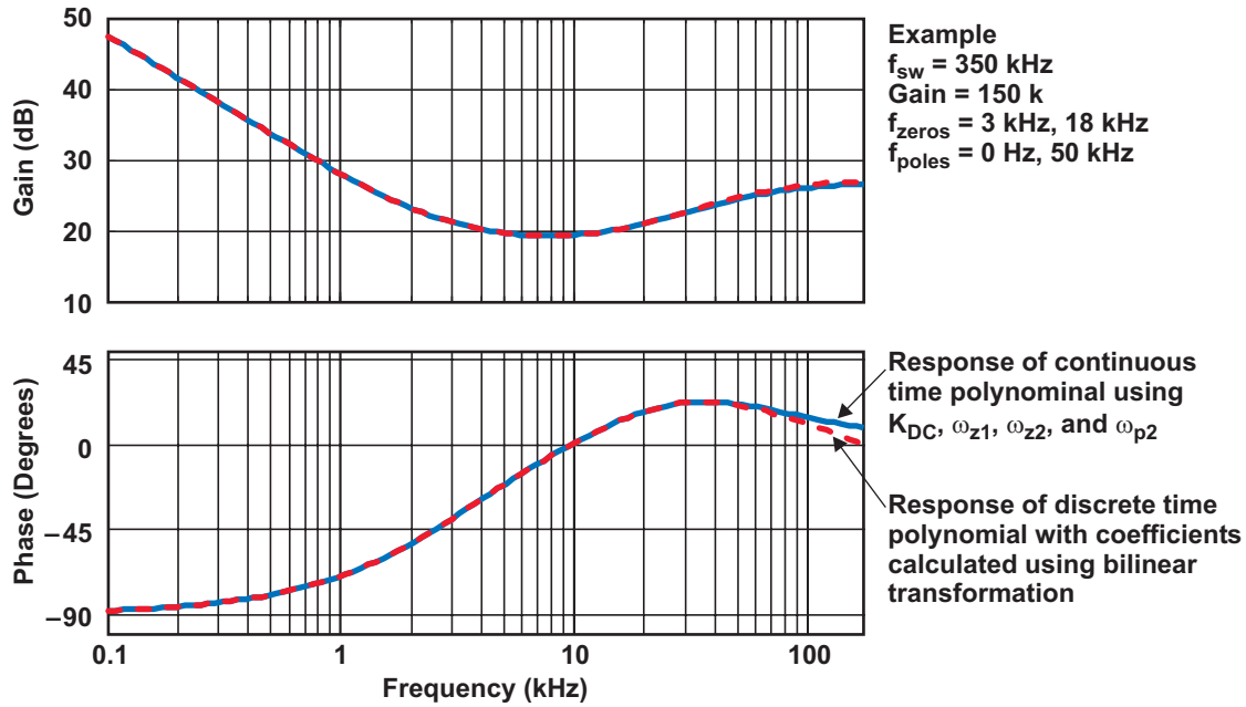
Fig. 12. Frequency response of continuous-time and discrete-time compensator.
