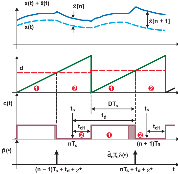
Fig. 6. Waveforms illustrating derivation of a discrete-time model for a digitally-controlled SMPS.
