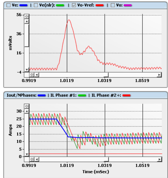
Fig. 35. Simulation results of a 50- to 25-A load transient for a synchronous two-phase buck converter.
