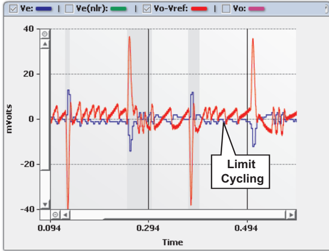
Fig. 25. Limit cycling with low nonlinear gain.
