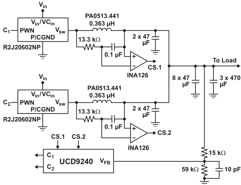
Fig. 29. Block diagram of a two-phase buck converter using the UCD9240 digital controller.
