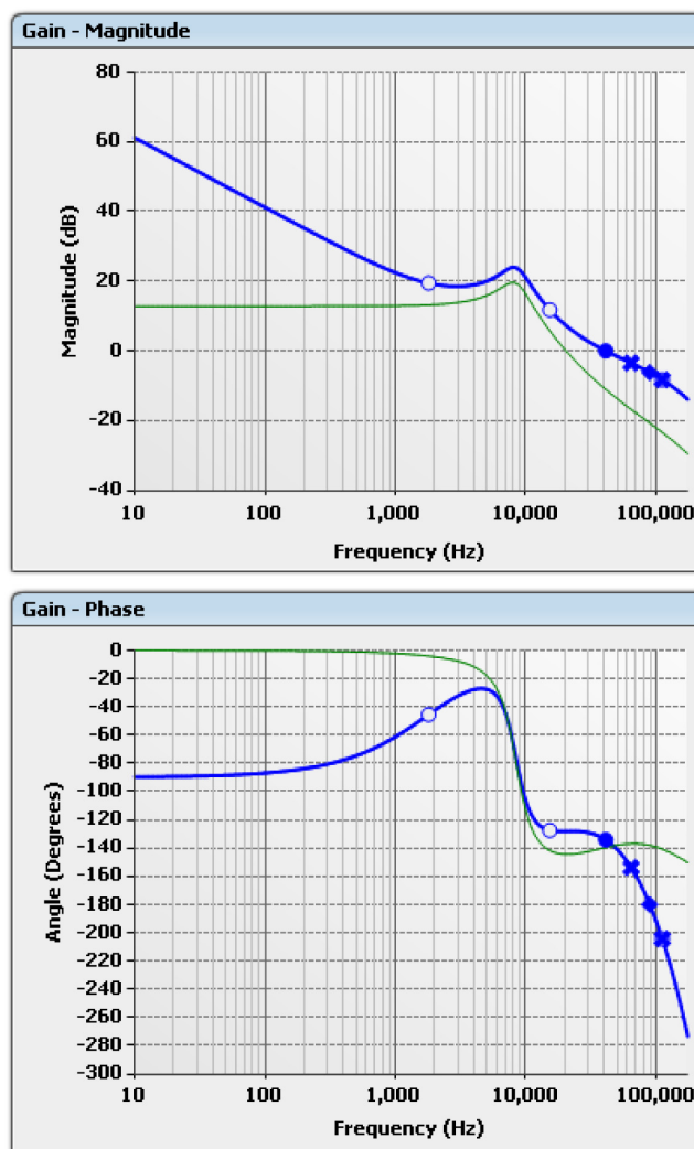
Fig. 32. Loop gain and control-to-output-voltage frequency response.
