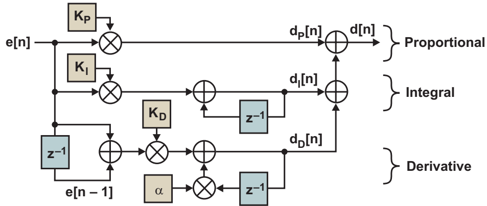
Fig. 11. PID digital-filter implementation.
