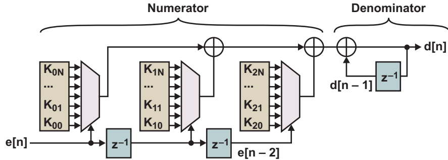
Fig. 9. Table look-up implementation of a digital filter.
