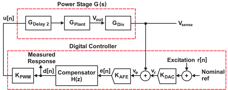
Fig. 26. The injection and measurement for system identification in the UCD9240.
