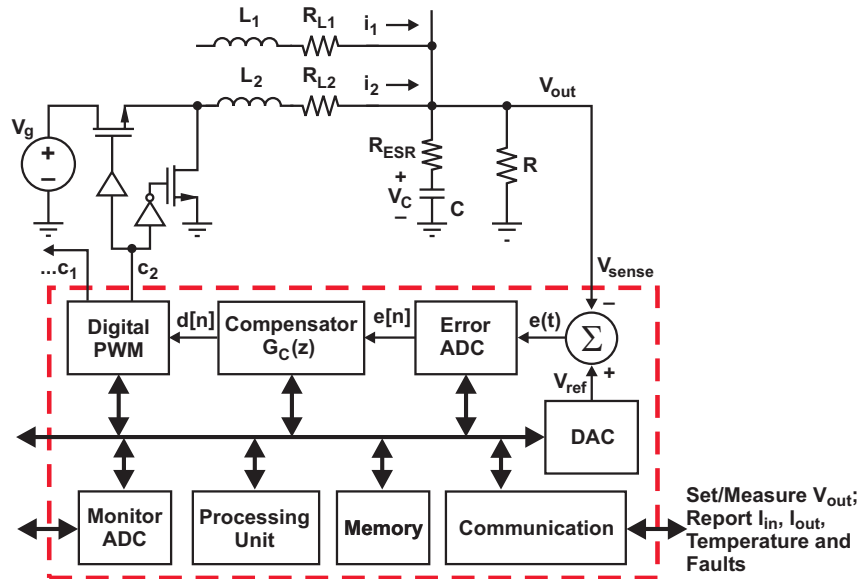
Fig. 2. Digital controller in an SMPS.
