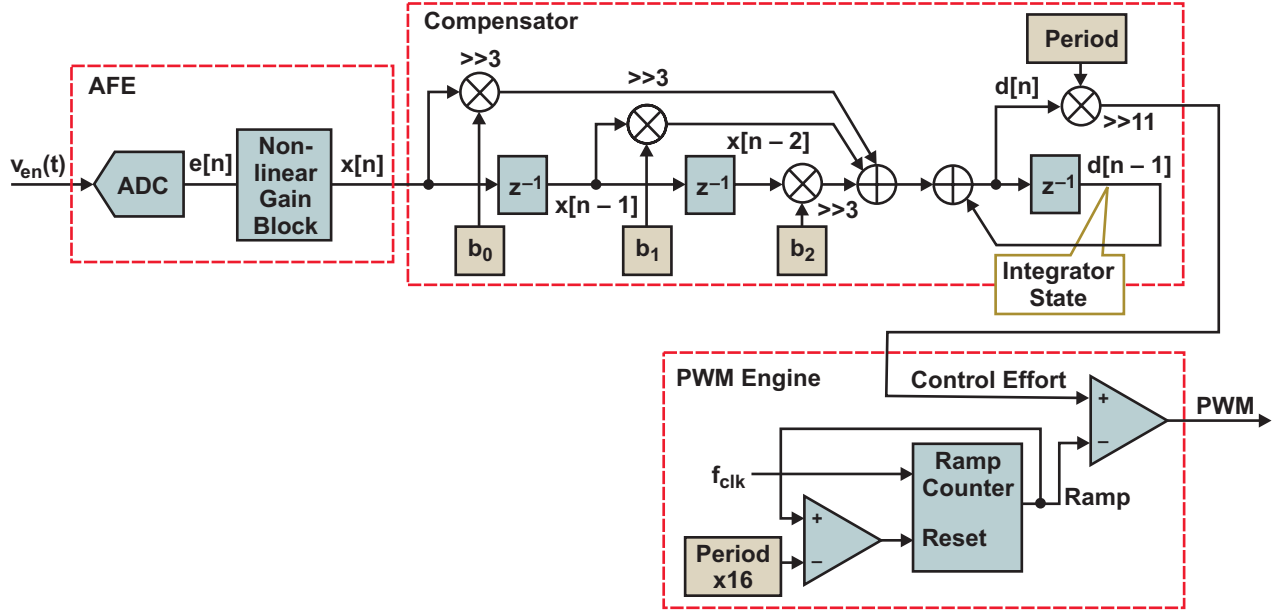
Fig. 24. Location of the integrator state in the controller system.
