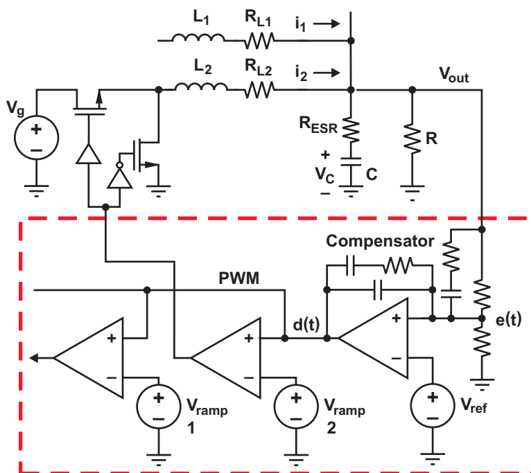
Fig. 1. Analog-controlled SMPS.
