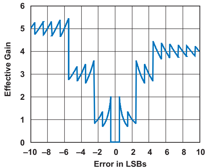
b. Gain with nonlinear gain applied.
