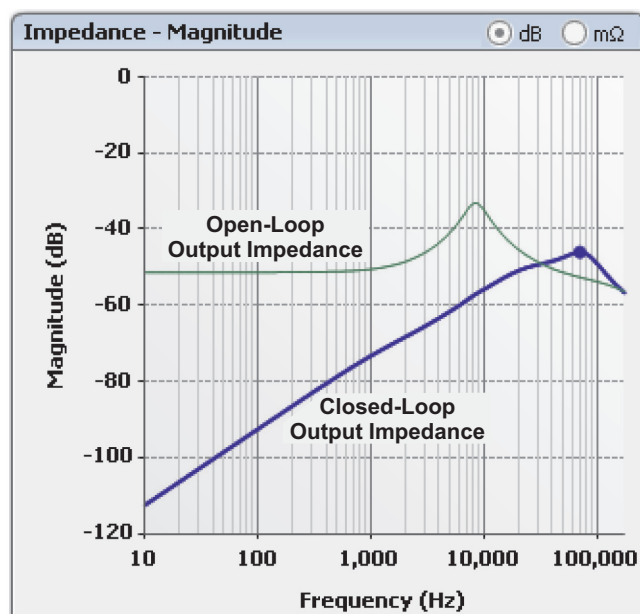
Fig. 33. Frequency response of open-loop and closed-loop output impedance.
