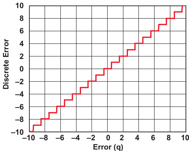
a. ADC in/out transfer function with quantization.
