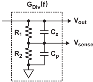
Fig. 8. Divider network.
