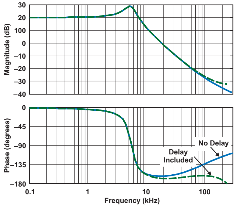
Fig. 7. The control-to-output-voltage magnitude and phase response of a buck converter.
