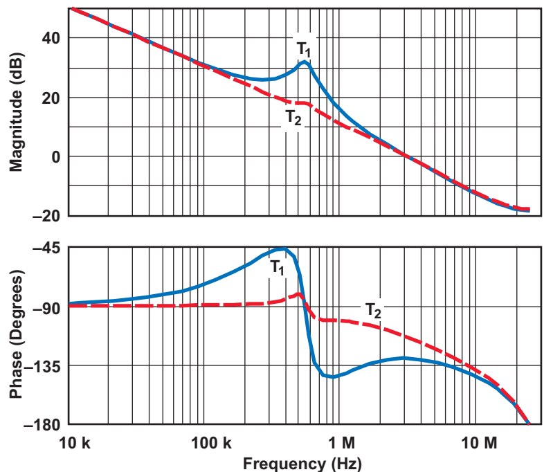
Fig. 13. The closed-loop gain of the buck converter with (1) real zeros and (2) complex zeros.
