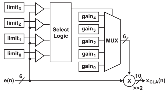
Fig. 19. Digital controller with nonlinear quantization.
