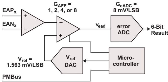
Fig. 17. Block diagram of an eADC together with a programmable DAC.
