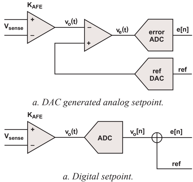
Fig. 16. Comparison of analog and digital setpoint reference.
