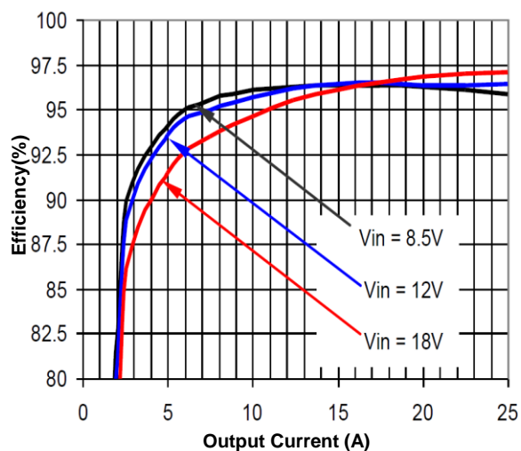
Figure 6(a). Efficiency vs. Load Current (25°C)
