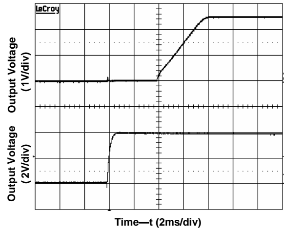
Figure 6. Start-Up from Application of Input Voltage (Input voltage 4V, Output current 20A)
