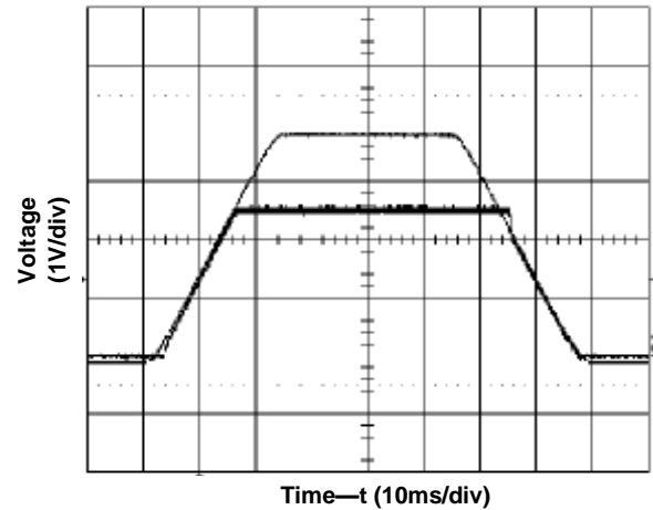
Figure 10. Voltage Tracking/Sequencing (with tracking option, V_{in} = 4V , V_o = 2.5V , I_o = 0A )
