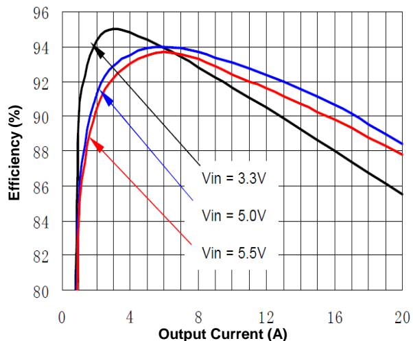
Figure 1(c). Efficiency vs. Load Current (25°C, 1.2V)
