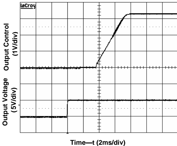
Figure 5. Start-Up from Enable Control (Input voltage 5V, Output current 20A)
