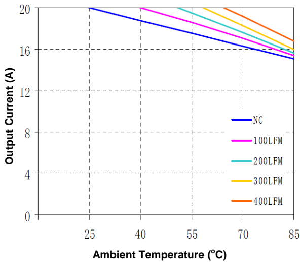
Figure 11(e). Current Derating Curve for 2.5V Output (Vin = 5V open frame)
