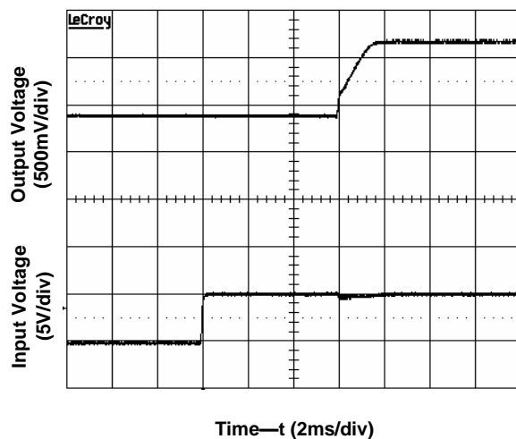
Figure 2. Start-Up with Prebias (Input voltage 5V, Output current 0A, Output voltage 1.8V, Prebias 1.2V)
