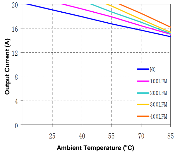
Figure 11(f). Current Derating Curve for 3.3V Output (Vin = 5V open frame)
