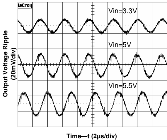
Figure 3. Output Ripple Voltage at 2.5V, 20A Output
