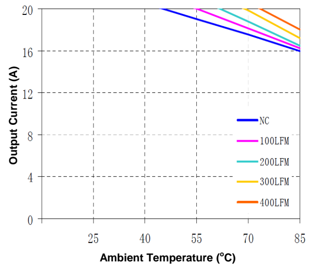
Figure 11(b). Current Derating Curve for 1.2V Output ( V_{in} = 5V open frame)
