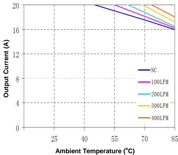
Figure 11(a). Current Derating Curve for 1.0V Output ( V_{in} = 5V open frame)
