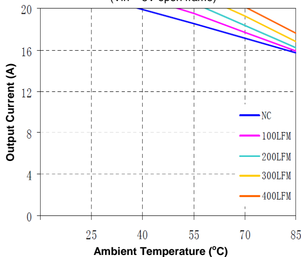
Figure 11(c). Current Derating Curve for 1.5V Output ( V_{in} = 5V open frame)
