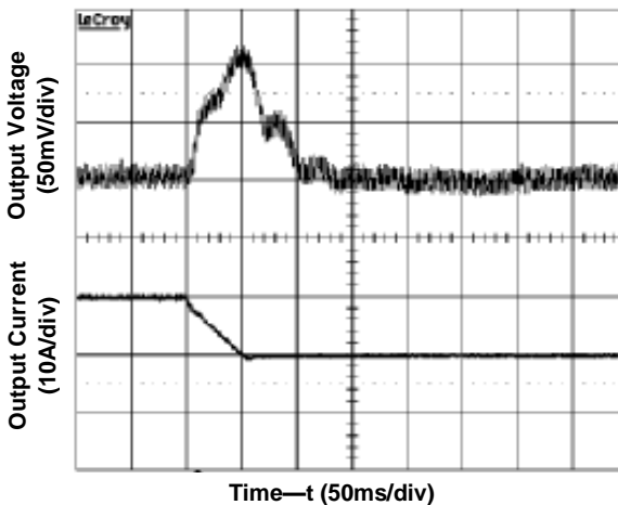
Figure 7. Transient Load Response (Input voltage 5V, Output current 20→10A, Slew rate 0.2A/μs)
