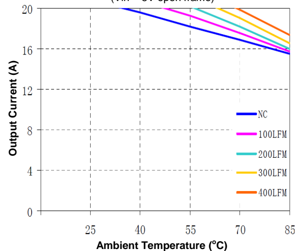
Figure 11(d). Current Derating Curve for 1.8V Output ( V_{in} = 5V open frame)
