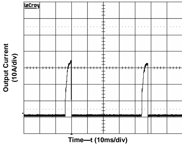
Figure 9. Short Circuit Current ( V_{in} = 5V )
