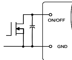
Figure 12. Circuit for Positive Logic Control
