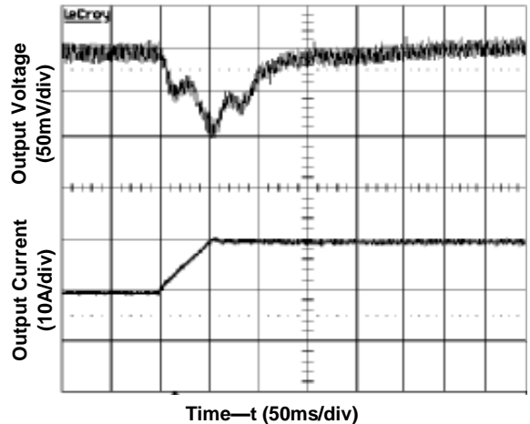
Figure 8. Transient Load Response (Input voltage 5V, Output current 20→10A, Slew rate 0.2A/μs)
