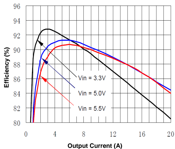
Figure 1(a). Efficiency vs. Load Current (25°C, 0.8V)
