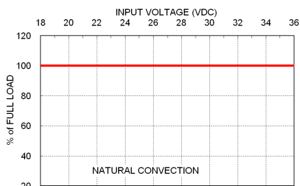
PDL09-24S12M Load Derating v.s. Input Voltage (at T_a = 60^\circ\text{C} )
