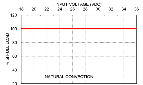
PDL09-24S12 Load Derating v.s. Input Voltage (at T_a = 55^\circ\text{C} )
