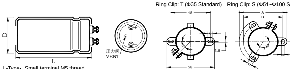
Ring Clip Dimensions:
